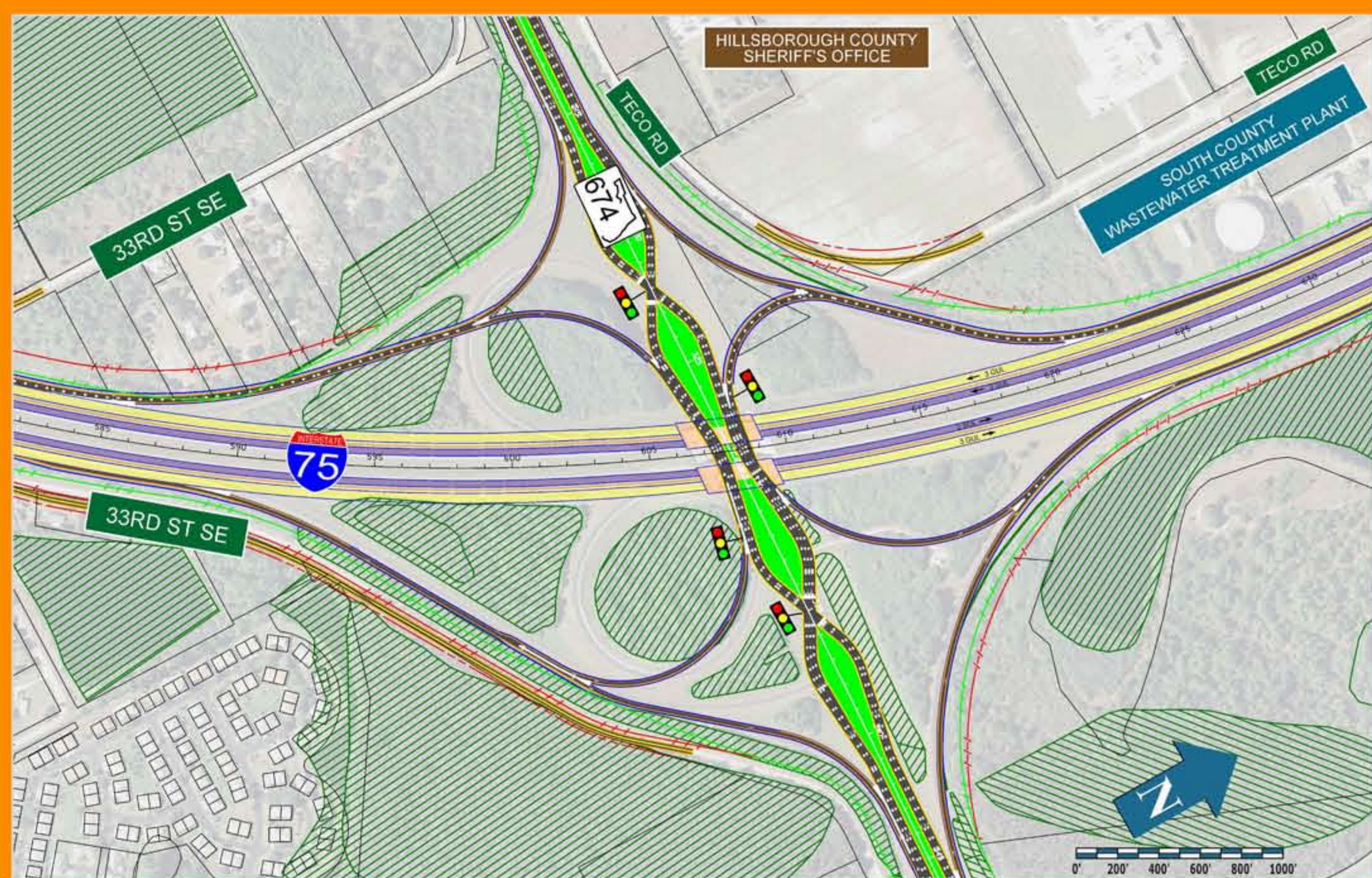
Option A - Diverging Diamond
