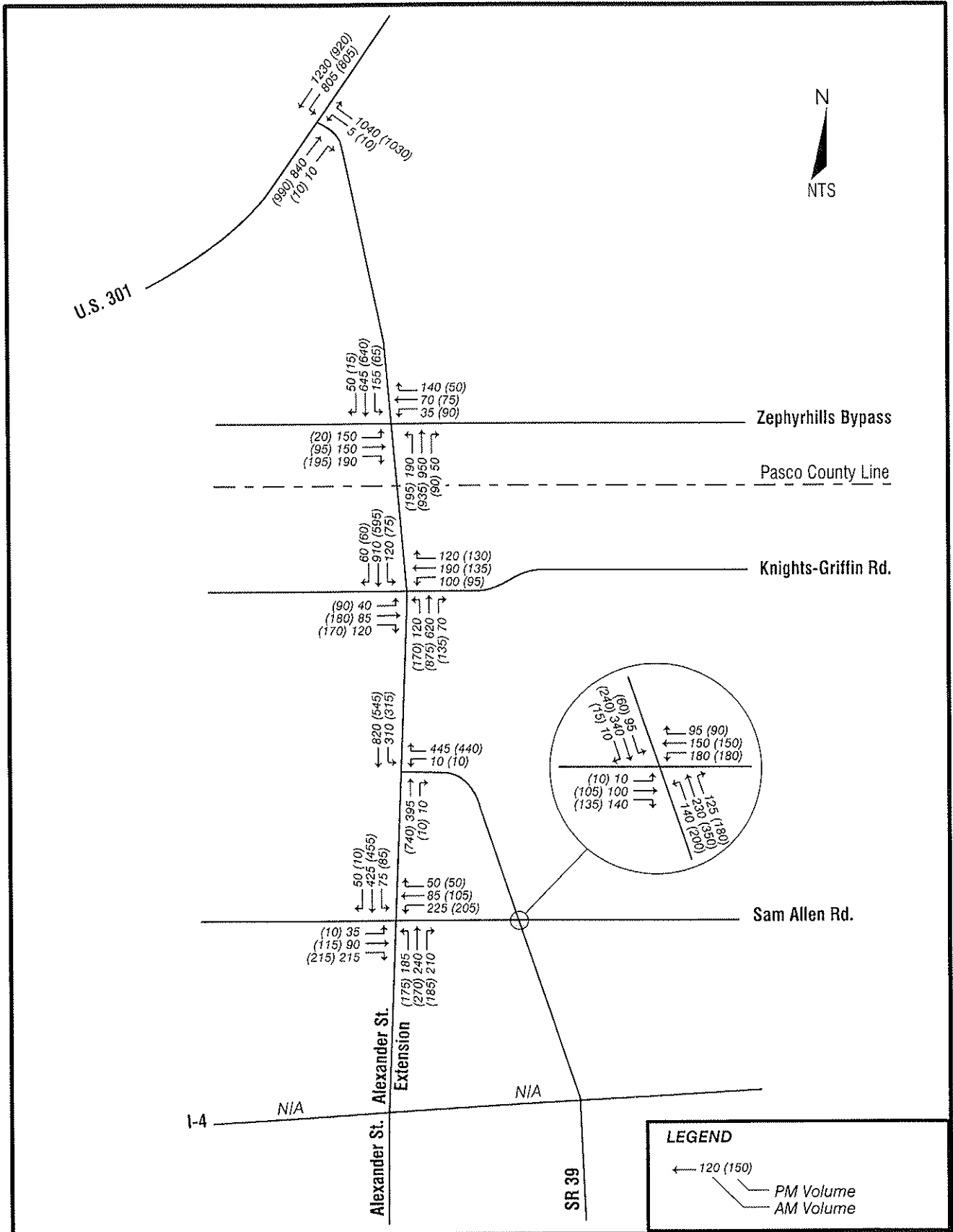
YEAR 2020 BUILD TURNING MOVEMENT VOLUMES S.R. 39 FROM I-4 TO U.S. 301 WPI SEGMENT No. 255099 1 & 256289 1 FAP No. F-321-1(4) HILLSBOROUGH AND PASCO COUNTIES, FLORIDA
