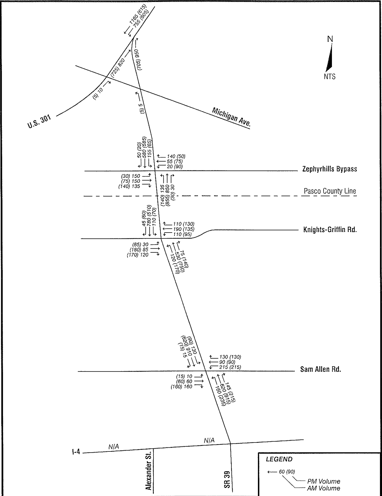
STATE OF FLORIDA DEPARTMENT OF TRANSPORTATION YEAR 2020 NO BUILD TURNING MOVEMENT VOLUMES S.R. 39 FROM I-4 TO U.S. 301 WPI SEGMENT No. 255099 1 & 256289 1 FAP No. F-321-1(4) HILLSBOROUGH AND PASCO COUNTIES, FLORIDA Figure 3-11
