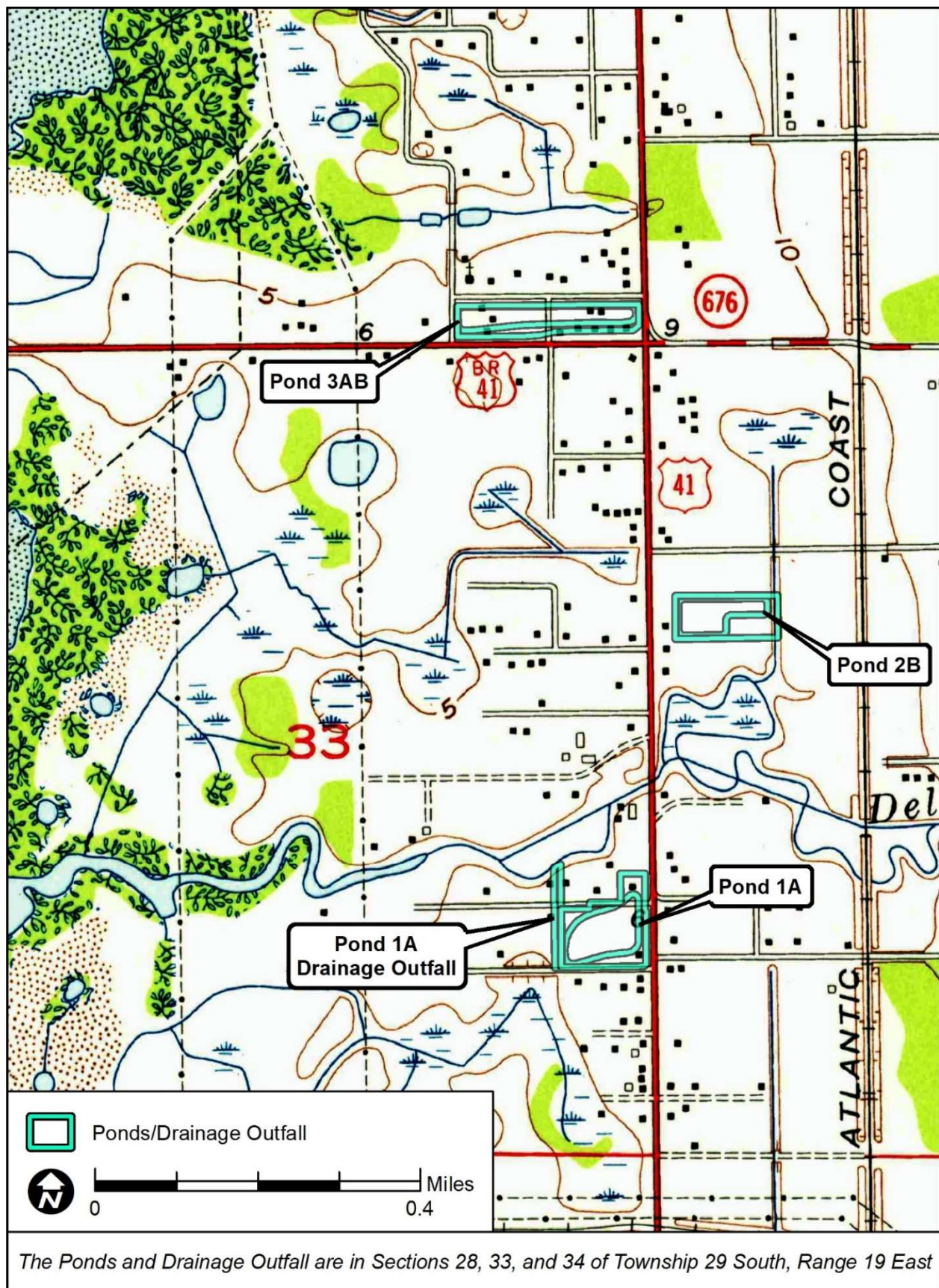
Figure 4-7 Ponds and Drainage Outfall on the Tampa (1956) USGS Quadrangle Map
