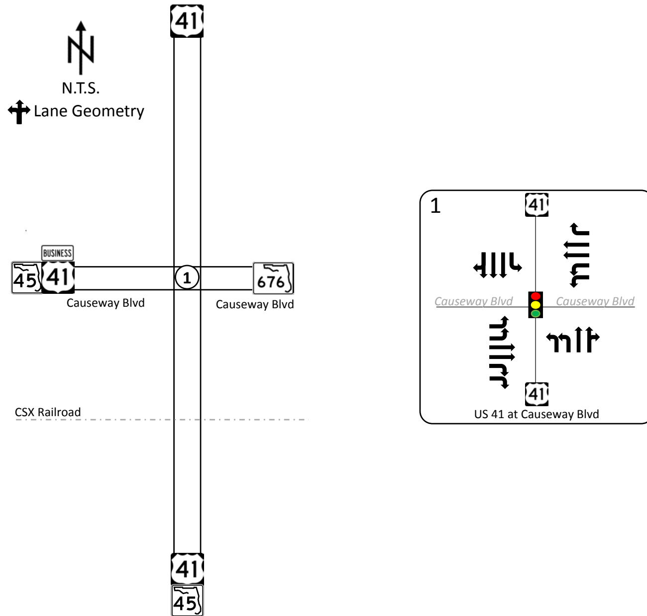
Figure 5.1. Existing Lane Configurations
