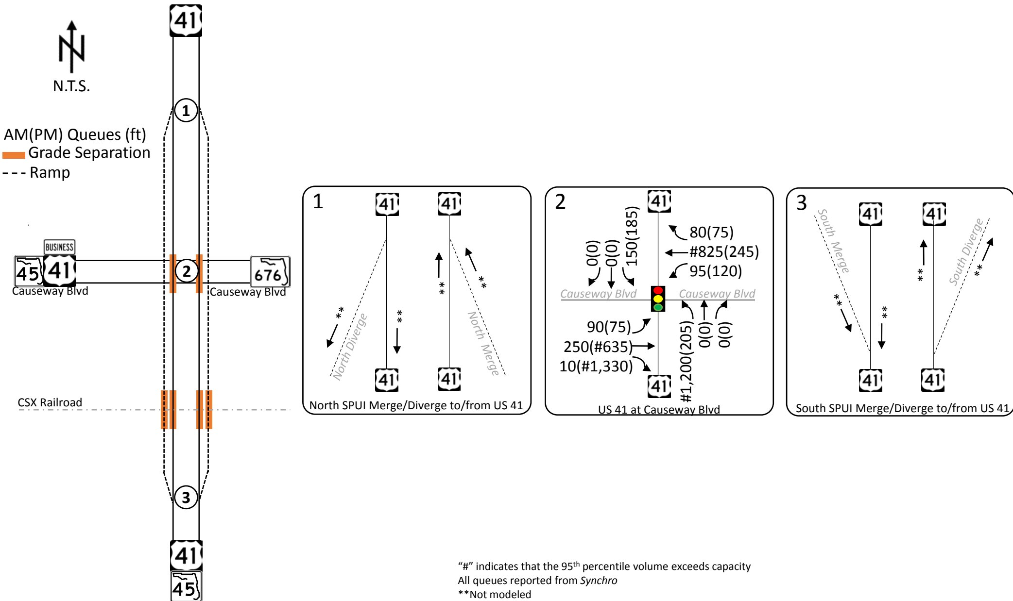
Figure 7.9. Build Alternative 4 Design Year 95 th Percentile Queues
