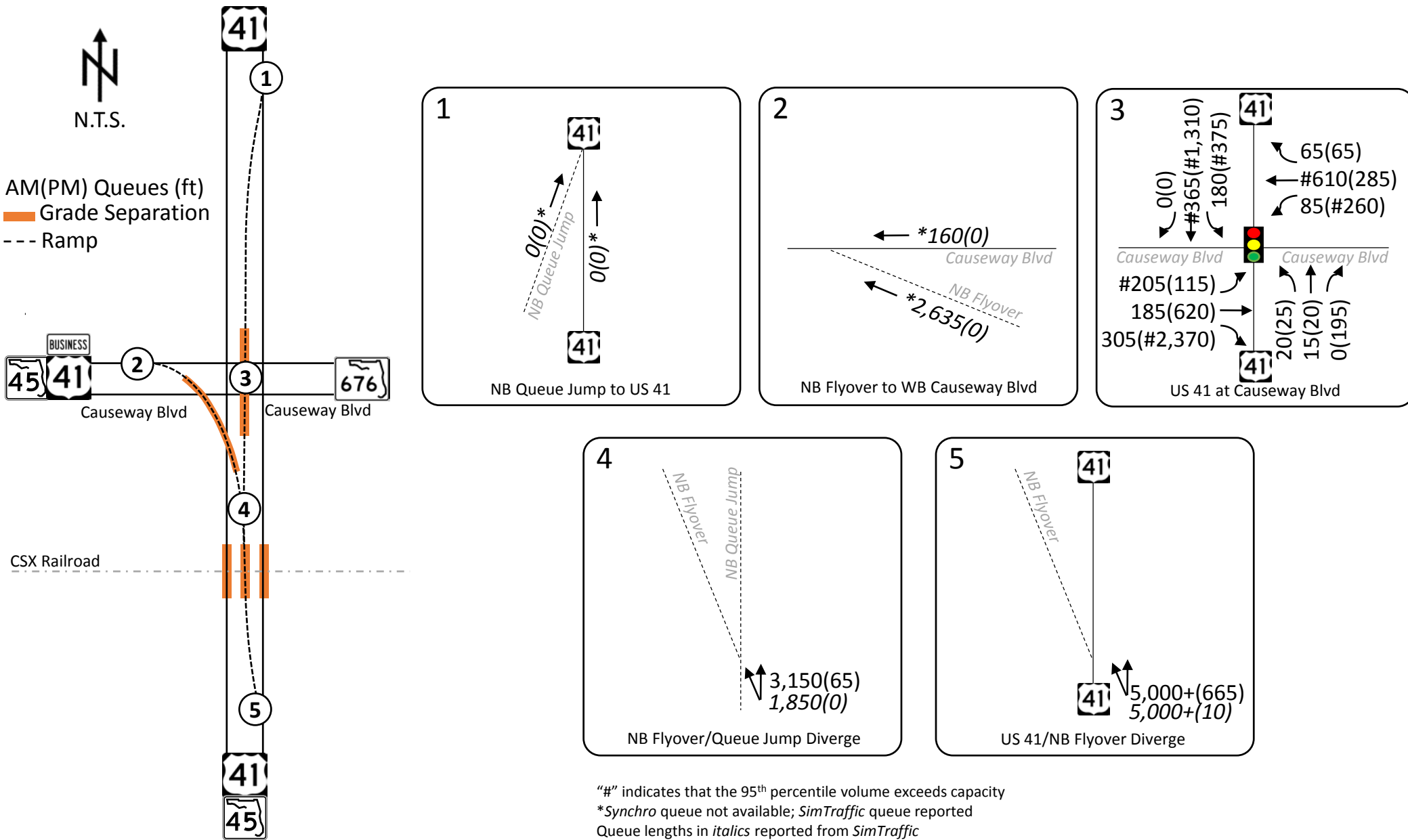
Figure 7.3. Build Alternative 1 Design Year 95 th Percentile Queues
