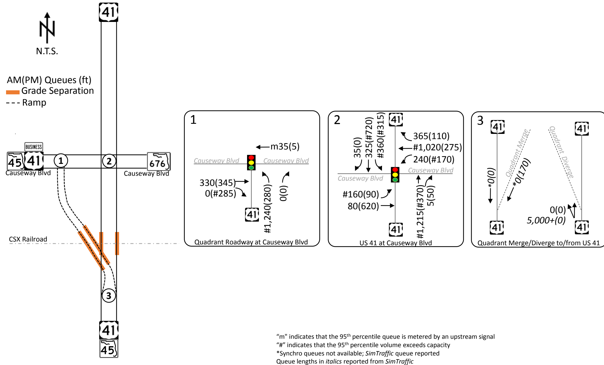
Figure 7.5. Build Alternative 2 Design Year 95 th Percentile Queues
