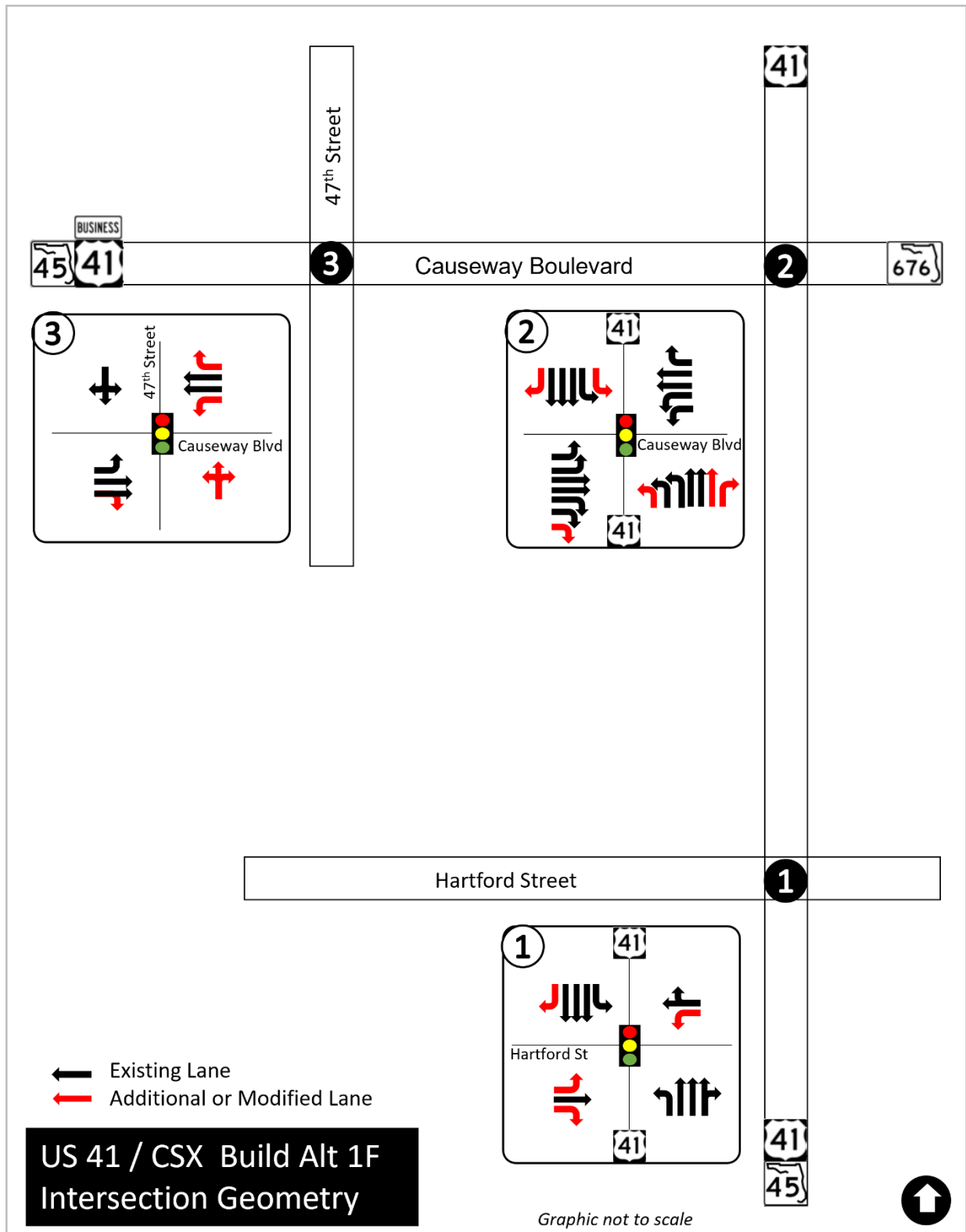
Figure 3.1. Alternative 1F Lane Configuration
