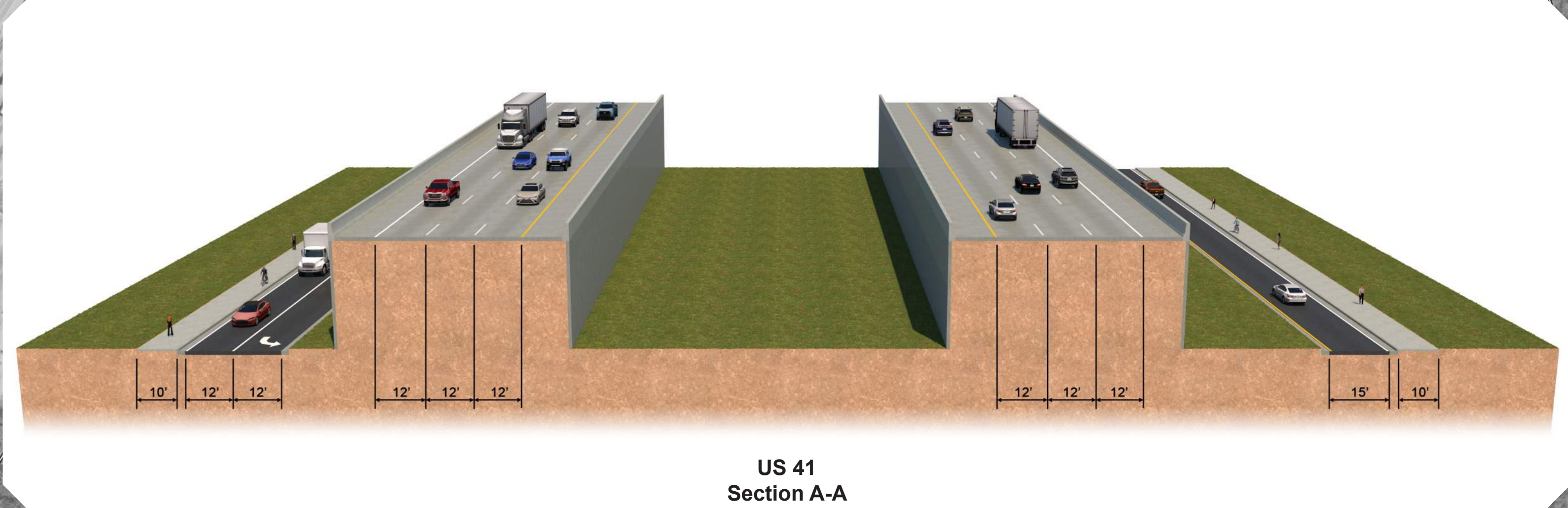
US 41 Section A-A
