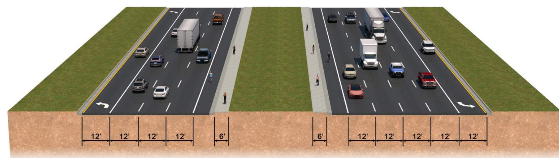
Causeway Boulevard Section B-B
