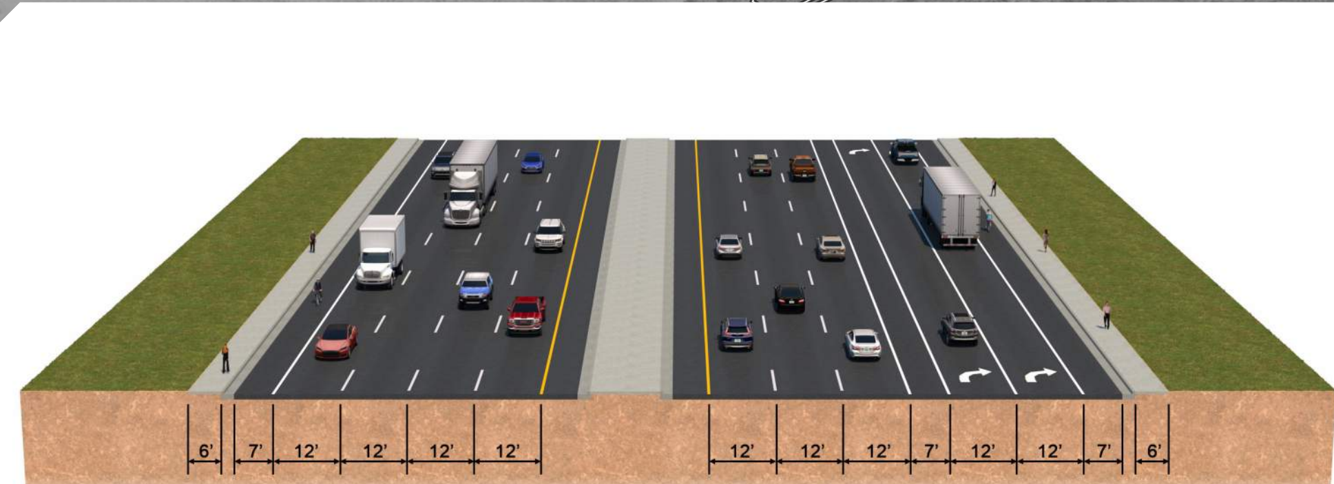
Causeway Boulevard Section C-C
