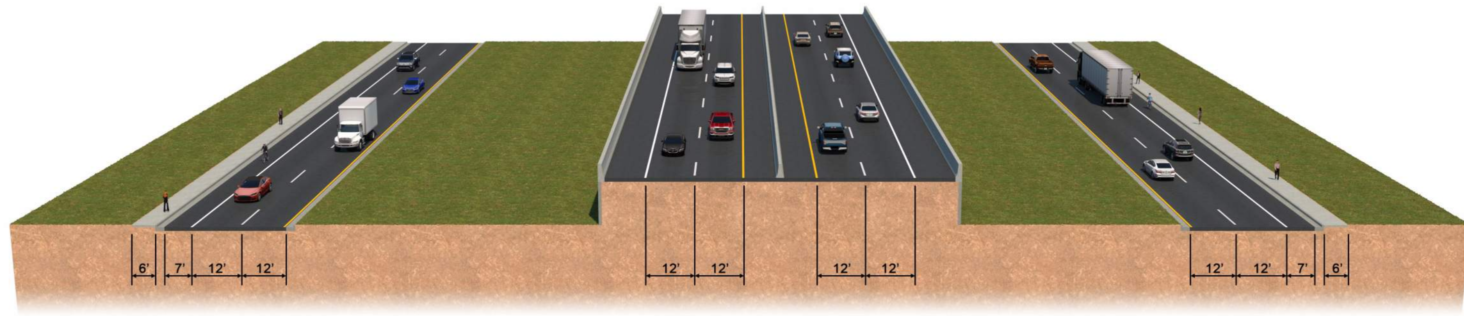
US 41 Section D-D
