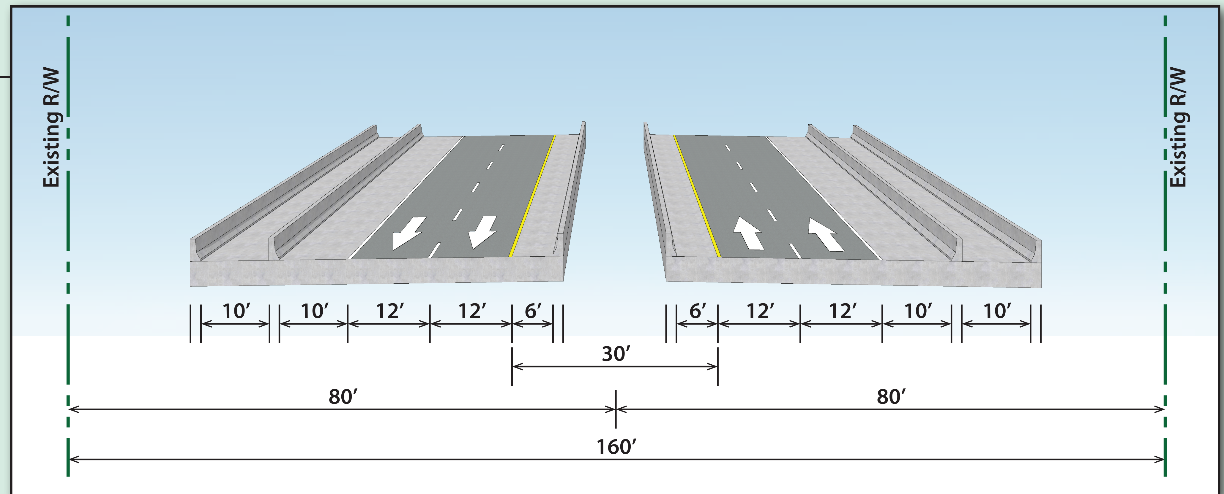
US 98 over the Hillsborough River & US 98 over Old Lakeland Highway/CSX Railroad
